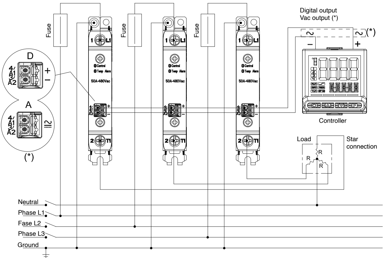
Three-phase Wye connection with neutral - GRS-H with V DC command input ("D" type input)
